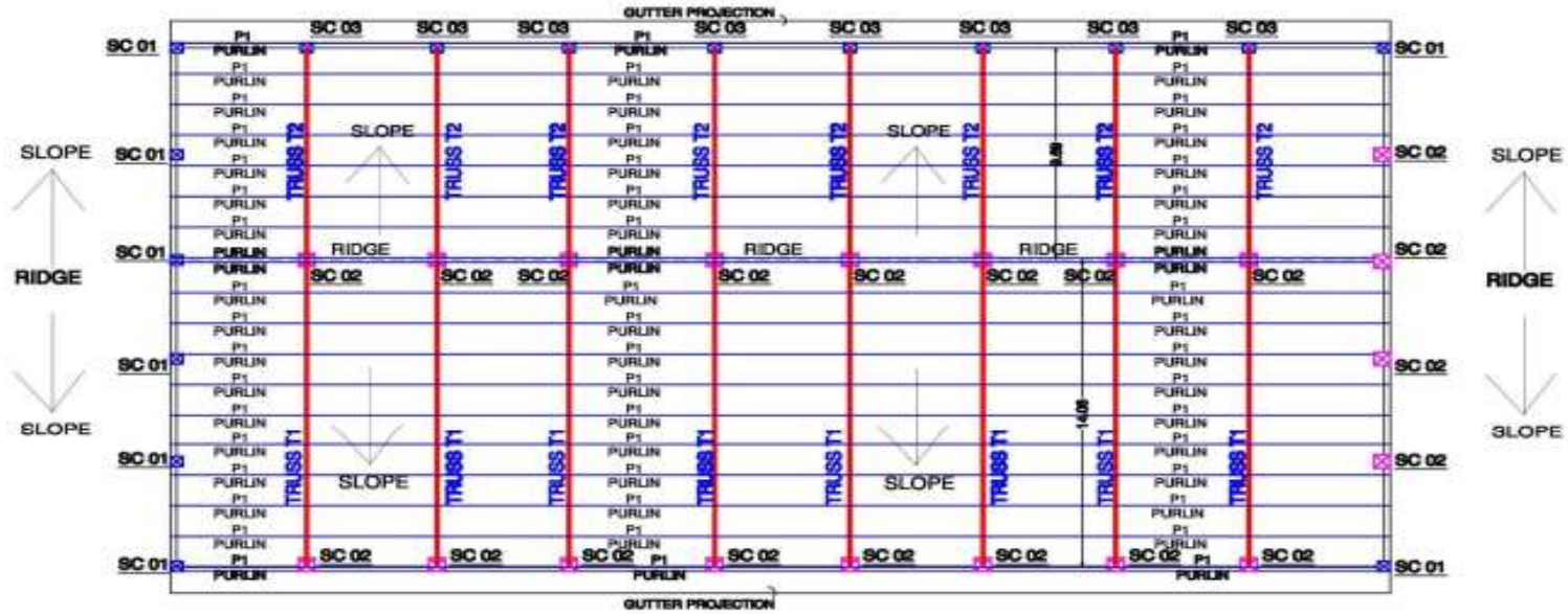
STRUCTURAL KEY PLAN @ ROOF LVL.
